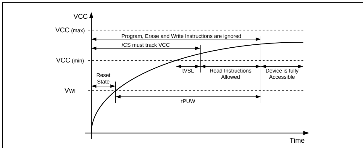
Figure 37a. Power-up Timing and Voltage Levels
